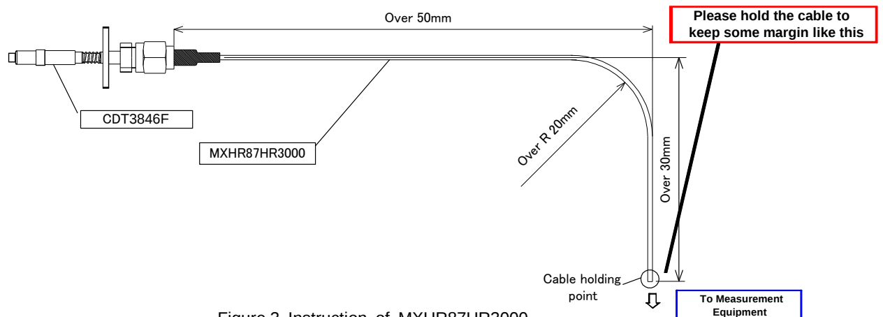
Figure.3 Instruction of MXHR87HR3000
