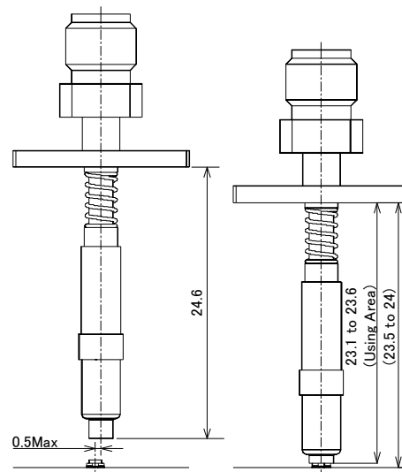
Figure.4 Acceptable engagement range to MM8930-2620
