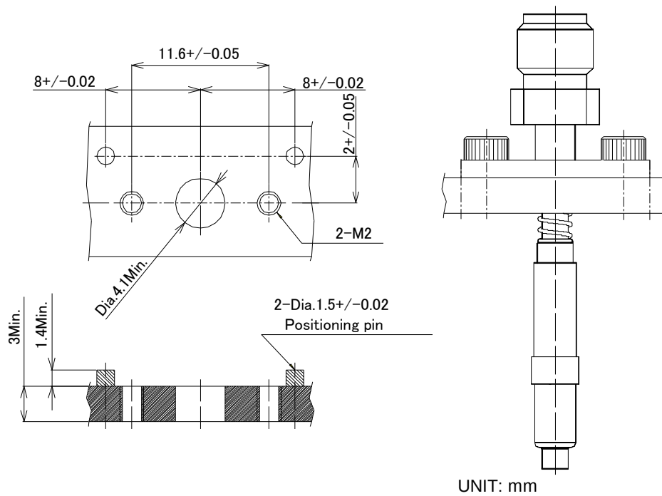
Figure.5 Machine's hole diameter for attachment probe
