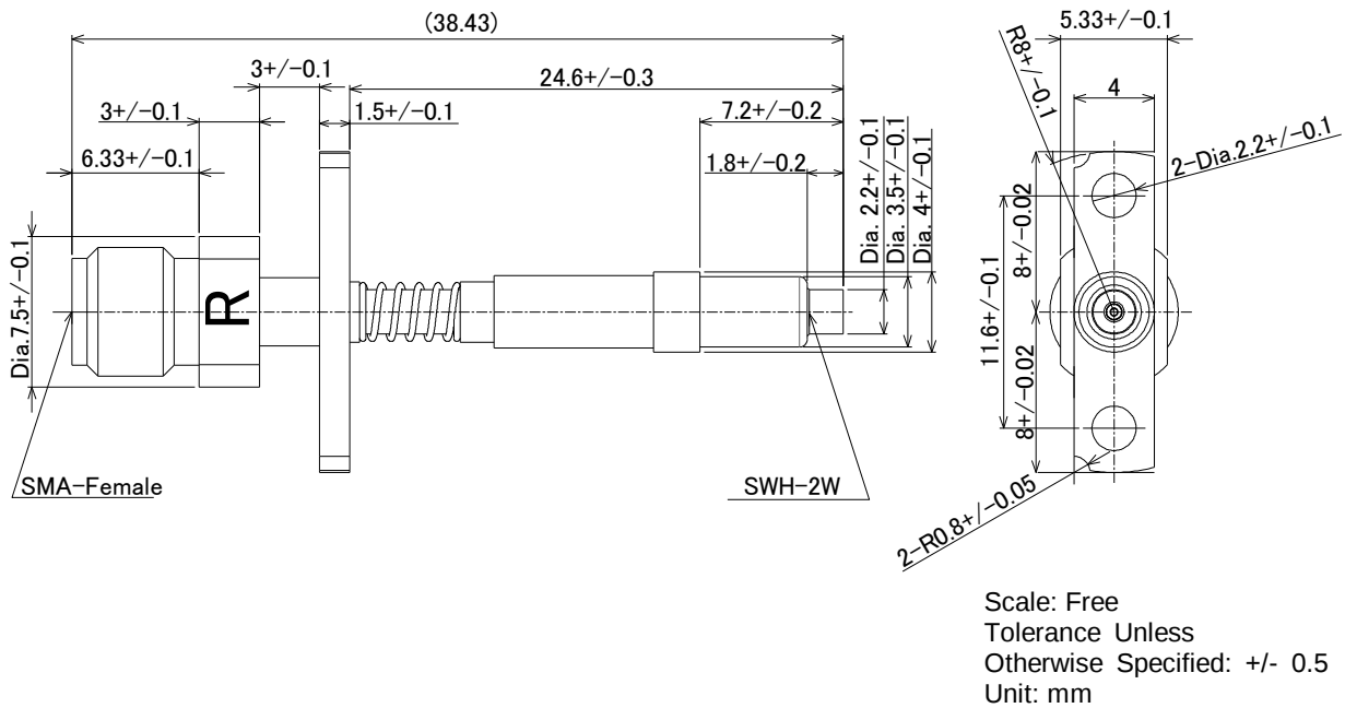
Figure 1 Construction
